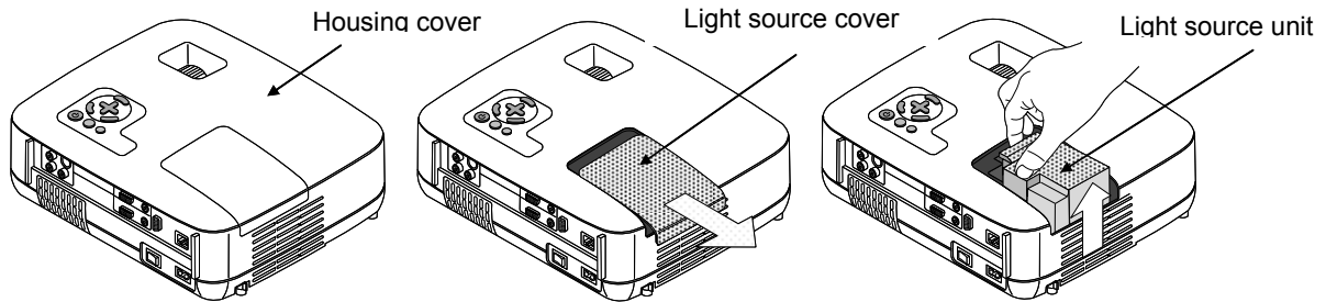
Figure 1 – Protective housing and light source unit of a projector
