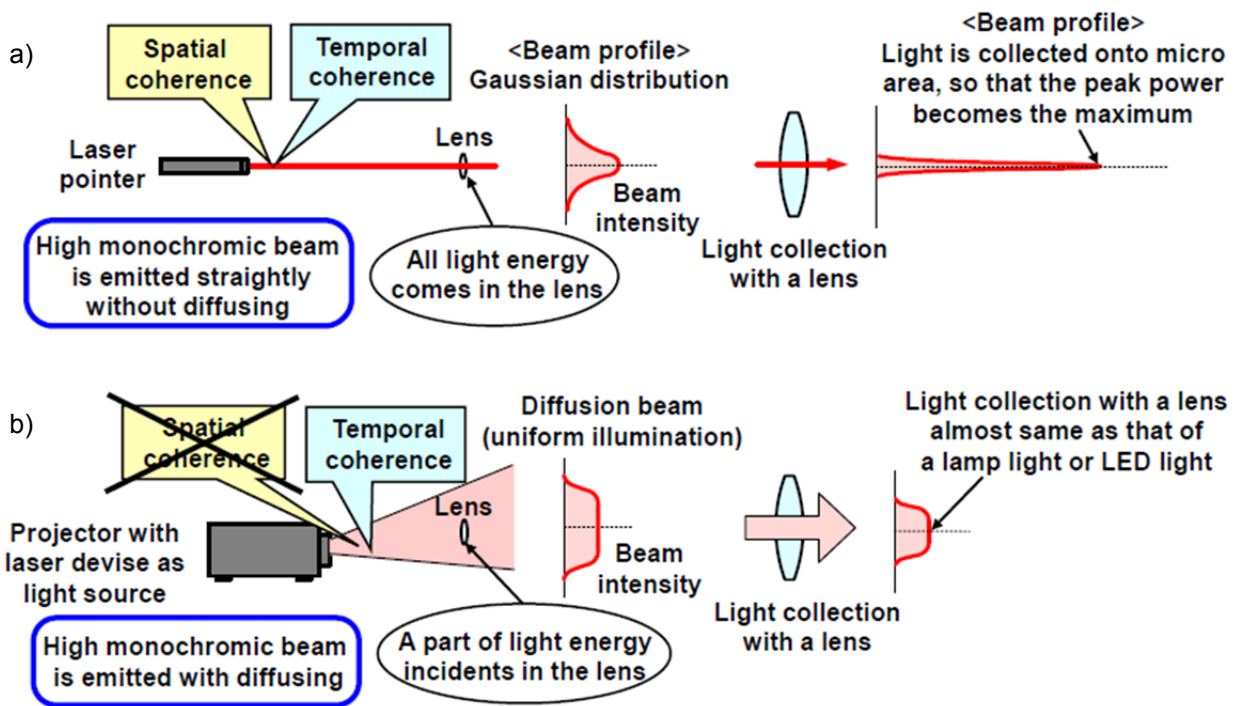
Figure 3 – Light-collection difference between a laser pointer and projector with laser device as light source
